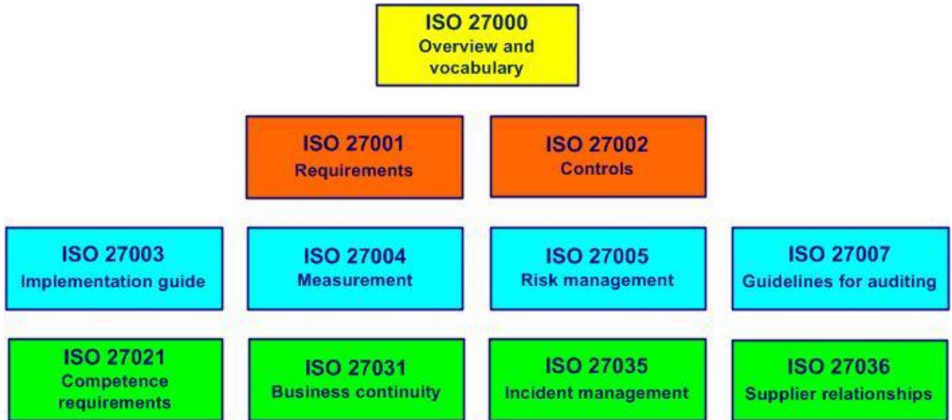
Figure 2-1. ISO 27000 family
